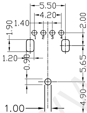
RECOMMEND PCB LAYOUT
